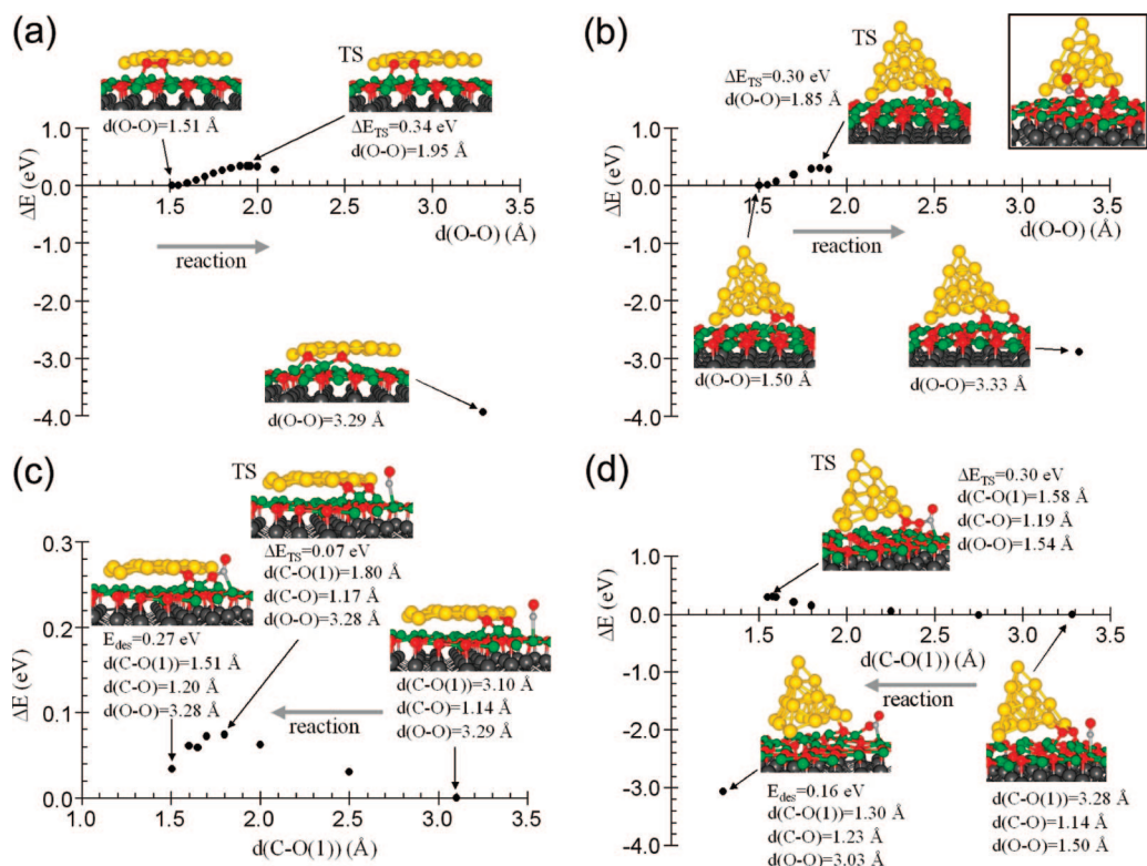
Figure 4. (a and b) Reaction paths for the dissociation of \text{O}_2 on 2D and 3D (tetrahedral) \text{Au}_{20} adsorbed on a one-layer thin MgO film supported on Mo(100). In both cases, the TS activation energy is relatively low: \Delta E_{\text{TS}} = 0.34 eV for the 2D gold structure (a) and \Delta E_{\text{TS}} = 0.30 eV for the 3D adsorbed cluster (b). In the inset to frame b, we show the relaxed structure of the adsorbed \text{CO}_2 molecule produced by the reaction of the dissociated \text{O}_2 molecule on \text{Au}_{20}(\text{T})/\text{MgO}(1\text{ L})/\text{Mo} with CO; no energy barrier is involved in this reaction, which starts from the dissociated \text{O}_2 molecule and a CO adsorbed on the MgO surface (on top of a Mg atom, with an adsorption energy of 0.55 eV), at a distance of 2.48 Å between the C atom and the closest dissociated O atom. The desorption energy of the product \text{CO}_2 is 0.31 eV. This reaction contributes to the low-temperature peak shown in Figure 1b–d. In parts c and d, we display two other low-temperature reactions pathways. The reaction in part c corresponds to an adsorbed planar, \text{Au}_{20}(\text{P}) cluster, and it starts from the adsorbed dissociated \text{O}_2 molecule shown in part a (with a dissociation activation energy of 0.34 eV) and a CO molecule adsorbed on top of a Mg atom [ E_{\text{B}}(\text{CO}) = 0.47 eV]. The generation of adsorbed \text{CO}_2 entails a TS barrier of E_{\text{TS}} = 0.07 eV and a desorption energy of the product E_{\text{des}}(\text{CO}_2) = 0.27 eV. The reaction in part d corresponds to an adsorbed 3D \text{Au}_{20}(\text{T}) cluster, and it involves a peripherally adsorbed activated \text{O}_2 molecule and a CO molecule adsorbed on the MgO surface ( E_{\text{B}} = 0.41 eV). The reaction in part d entails a TS barrier \Delta E_{\text{TS}} = 0.30 eV, and the desorption energy of the product is E_{\text{des}}(\text{CO}_2) = 0.16 eV. Color designation (online): Mg atoms in green, O atoms in red, Au atoms in yellow, C atoms in light gray, and Mo atoms in dark gray.
