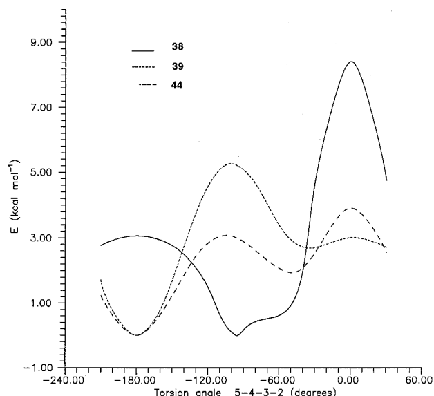
Figure 3. Computed energies of the vinylallenes 38 , 39 , and 44 as functions of the torsion angle \text{C}_2\text{C}_3\text{C}_4\text{C}_5 .
