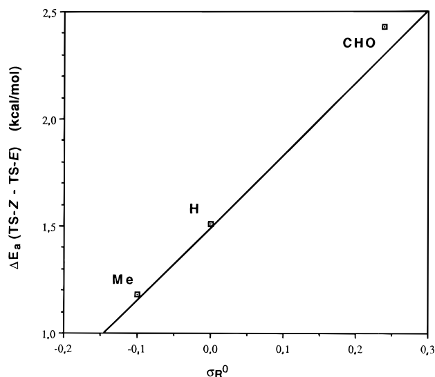
Figure 6. Plot of \Delta E_a versus \sigma_R^0 for the electrocyclic ring closures of substituted divinylallenes to alkylidenecyclobutenes.
