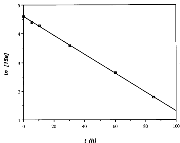
Figure 1. Plot of \ln [15a] versus time for the rearrangement of 15a to 30a in C 6 D 6 at 90 °C ([ 15a ] measured by monitoring the 1 H NMR signals attributed to H 6 of the reactant and H 1' of the product). Assuming irreversible first-order kinetics, this plot implies a half-life of 21.16 h and a rate constant k = 3.27 \times 10^{-2} \text{ h}^{-1} .
