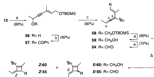
Scheme 9 a
