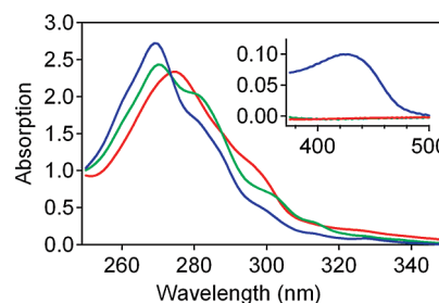
Figure 9. Reaction of 1 with \text{CH}_3\text{NC} followed by absorption spectroscopy. Electronic absorption spectra of 1 (36 \mu\text{M} in \text{CH}_2\text{Cl}_2 ) titrated with \text{CH}_3\text{NC} . The spectra obtained after addition of 0 (red solid line), 1 (green solid line) and 6 (blue solid line) equiv of \text{CH}_3\text{NC} are shown. Inset: the MLCT absorption of 1 .
