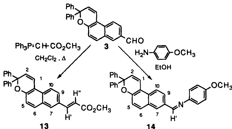
Scheme 9
