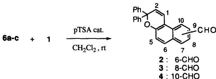
Scheme 4
