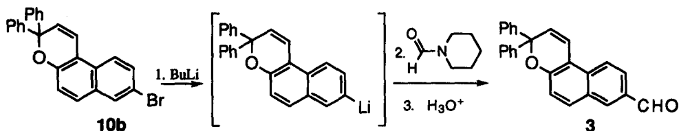
Scheme 7
