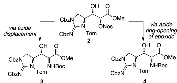
Scheme 1. Synthetic Strategy
