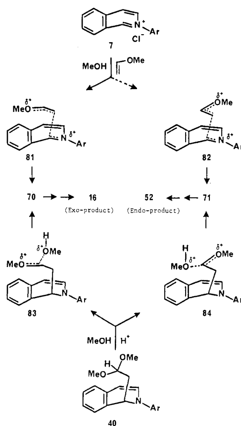
Scheme IX
