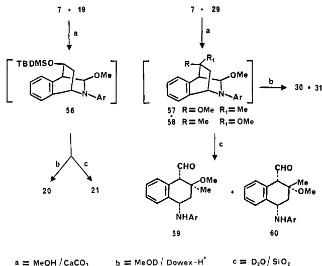
Scheme III
