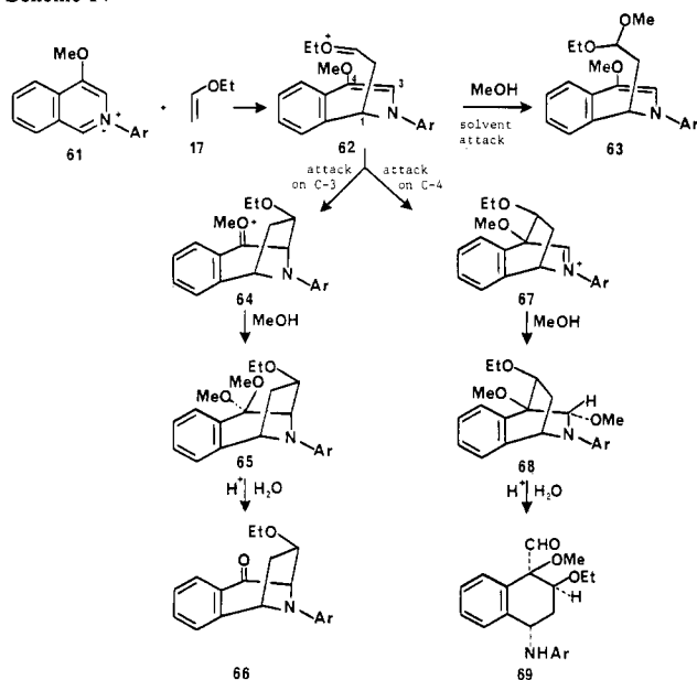
Scheme IV
