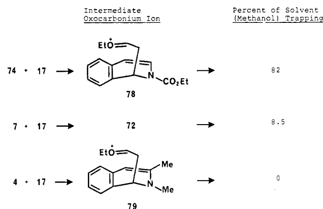
Scheme VII
