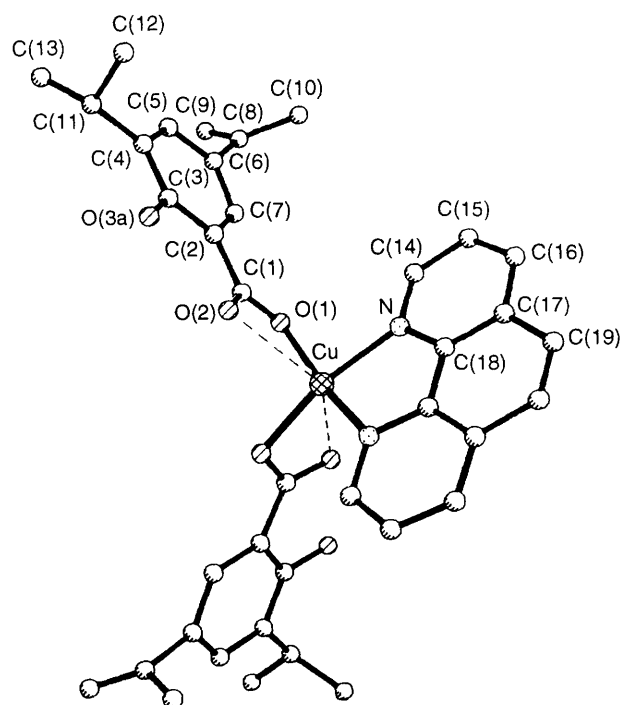
Fig. 1 The structure of [ \text{Cu}(\text{phen})(\text{Hdips})_2 ] 4 showing the numbering scheme. The hydroxyl group O(3a) is disordered 60:40 between C(3) and C(7) and is shown in the site of major occupancy
