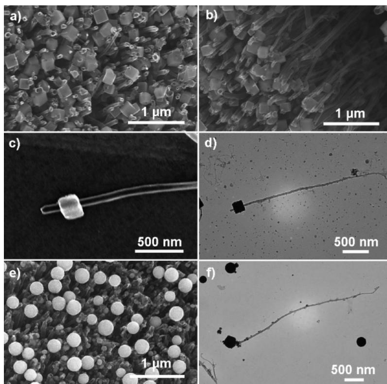
Figure 9. SEM (a–c) and TEM (d) images of Pt nanocubes deposited onto the nanotube tips by floating the Cu foil-supported aligned CNT films on an aqueous solution of 3.8 mM \text{K}_2\text{PtCl}_4 containing 5 mM \text{CuCl}_2 for 1 min. SEM (e) and TEM (f) images of Pt nanospheres deposited onto the nanotube tips by floating the Cu foil-supported aligned CNT films on an aqueous solution of 0.95 mM \text{K}_2\text{PtCl}_4 for 30 min.
