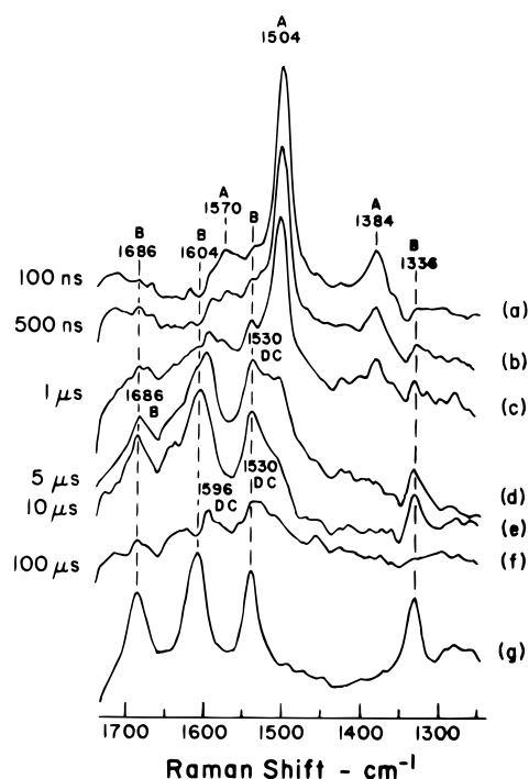
Figure 7. Raman spectra excited at 440 nm and observed (a) 100 ns, (b) 500 ns, (c) 1 \mu\text{s} , (d) 5 \mu\text{s} , (e) 10 \mu\text{s} , and (f) 100 \mu\text{s} after pulse irradiation of a \text{N}_2\text{O} -saturated 5 mM PABA solution containing 0.1 M \text{NaN}_3 at pH \sim 5.5 . (g) Spectrum taken at 1.0 \mu\text{s} after pulse irradiation of a \text{N}_2\text{O} -saturated aqueous solution of benzidine ( < 1 mM) and 0.1 M \text{NaN}_3 at pH \sim 5.9 .
