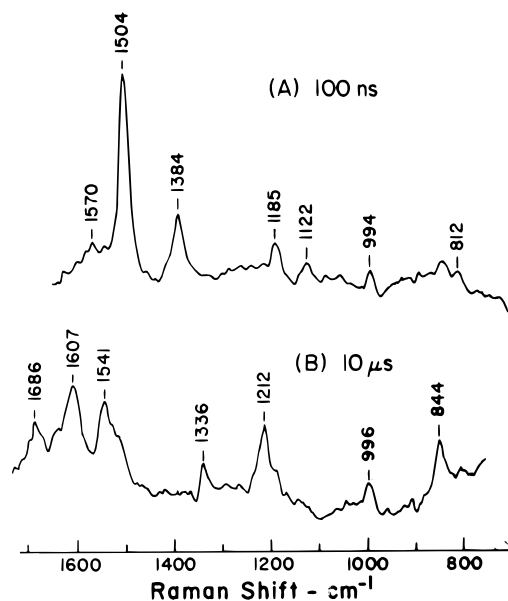
Figure 2. Resonance Raman spectra obtained (A) 0.1 and (B) 10 \mu s after electron pulse irradiation of \text{N}_2\text{O} -saturated aqueous solution containing 5 mM PABA, 0.1 M \text{NaN}_3 , and 2 mM phosphate buffer at pH 5.4. Excitation at 440 nm.
