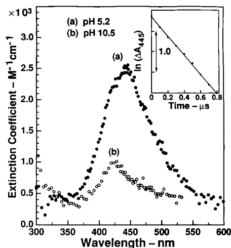
Figure 1. Transient absorption spectra obtained 2 \mu s after electron pulse irradiation of \text{N}_2\text{O} -saturated aqueous solution containing 1 mM PABA, 2 mM phosphate buffer, and 0.1 M \text{NaN}_3 at pH (a) 5.2 and (b) 10.5. The insert shows exponential decay of the 445-nm absorption peak in Figure 1a with time.
