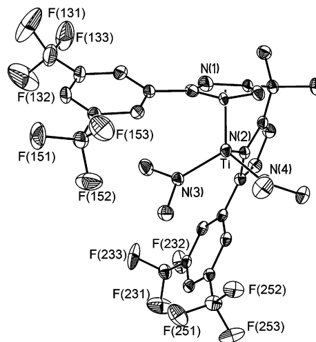
Figure 1. ORTEP structure from single-crystal X-ray diffraction on \text{Ti}(\text{NMe}_2)_2(\text{dmpm}^{3,5-\text{CF}_3}) (3). Selected bond distances (Å) and angles (deg): Ti–N(3) = 1.875(5), Ti–N(4) = 1.892(5), Ti–N(2) = 2.048(5), Ti–N(1) = 2.400(6); N(4)–Ti–N(3) = 107.1(2), N(4)–Ti–N(2) = 102.6(2), N(3)–Ti–N(2) = 104.8(2).
