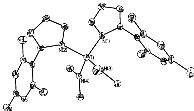
Figure 2. ORTEP structure from single-crystal X-ray diffraction on \text{Ti}(\text{NMe}_2)_2(\text{pyrr}^{\text{mes}})_2 ( 6 ). Selected bond distances (Å) and angles (deg): \text{Ti}-\text{N}(3) = 1.844(4) , \text{Ti}-\text{N}(4) = 1.865(4) , \text{Ti}-\text{N}(2) = 1.971(4) , \text{Ti}-\text{N}(1) = 2.007(4) ; \text{N}(3)-\text{Ti}-\text{N}(4) = 109.3(2) , \text{N}(3)-\text{Ti}-\text{N}(2) = 107.5(2) , \text{N}(4)-\text{Ti}-\text{N}(2) = 108.4(2) , \text{N}(3)-\text{Ti}-\text{N}(1) = 112.0(2) , \text{N}(4)-\text{Ti}-\text{N}(1) = 114.1(2) , \text{N}(2)-\text{Ti}-\text{N}(1) = 105.2(2) .
