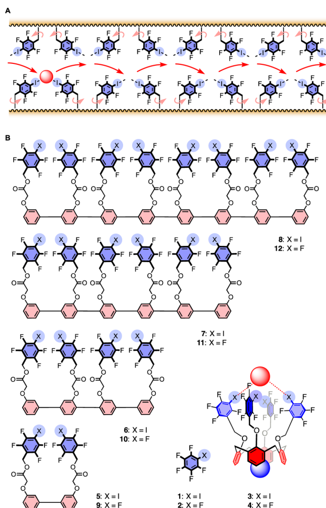
Figure 1. (A) Schematic representation of anion hopping along transmembrane halogen-bonding cascades. (B) Halogen-bond donors as monomers ( 1 ), 6 in cyclic arrays ( 3 ), 7 and in linear arrays ( 5 – 8 ), together with the controls for anion- \pi interactions ( 2 , 4 , 9 – 12 ).
