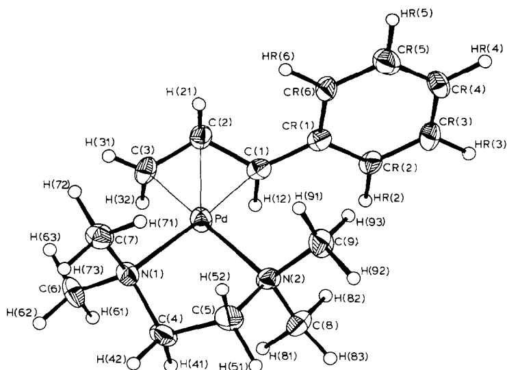
Fig. 1. Perspective view of the cation of [(\eta\text{-1-Ph-C}_3\text{H}_4)\text{Pd}(\text{tmeda})]\text{BF}_4 ( 4 ).
