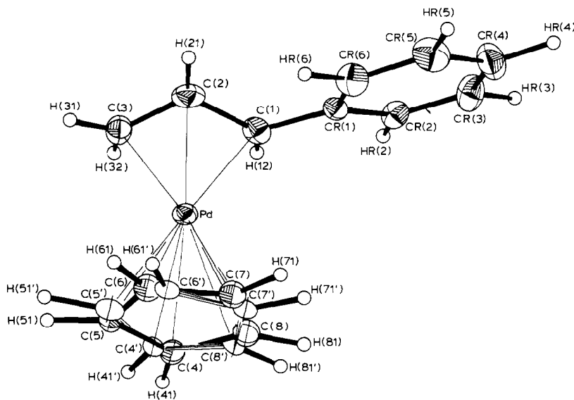
Fig. 2. Perspective view of [(\eta\text{-C}_5\text{H}_5)\text{Pd}(\eta\text{-1-Ph-C}_3\text{H}_4)] ( 5 ), showing both components of the disordered (\eta\text{-C}_5\text{H}_5) ligand.
