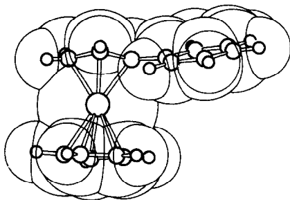
Fig. 5. The space filling diagram of 5 . For clarity only the major component of the (η-C 5 H 5 ) ligand is shown.
