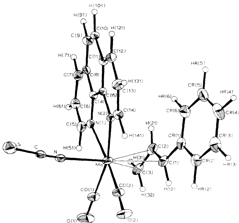
Fig. 3. Perspective view of [(\text{phen})\text{Mo}(\text{CO})_2(\text{NCS})(\eta\text{-}1\text{-Ph-C}_3\text{H}_4)] ( 8 ).
