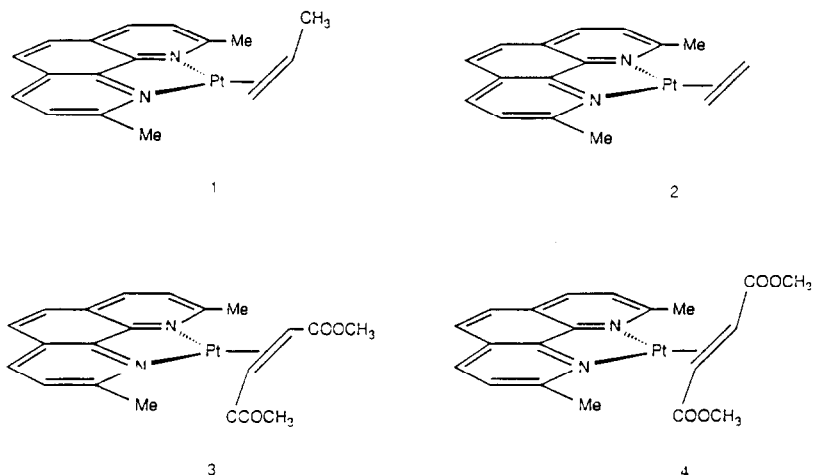
Fig. 1. Three-coordinate complexes used in this work. The organotin halides used are \text{SnR}_n\text{Cl}_{4-n} : \text{SnMe}_3\text{Br} , \text{SnMe}_3\text{Cl} , \text{SnMe}_2\text{Cl}_2 , \text{SnMeCl}_3 , \text{SnPh}_3\text{Cl} and \text{SnPh}_2\text{Cl}_2 .
