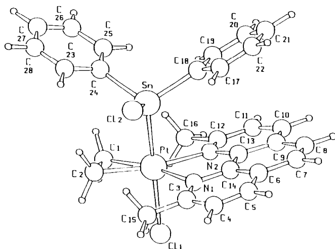
Fig. 2. View of the molecule [\text{Pt}(2,9\text{-Me}_2\text{-}1,10\text{-phen})\text{Cl}(\text{SnPh}_2\text{Cl})(\text{C}_2\text{H}_4)] .
