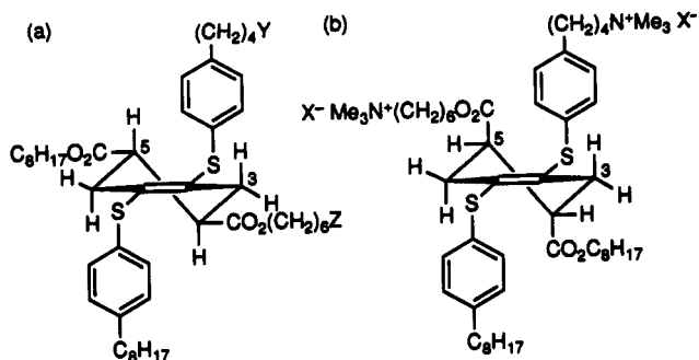
Figure 3. (a) Half-chair conformation of 16c (Y = Z = N + Me 3 X - ) and 19c (Y = OH; Z = Br) with trans diequatorial ester groups. (b) Half-chair conformation of 17c with trans diaxial ester groups.
