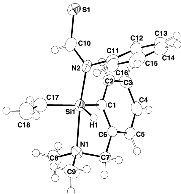
Fig. 1. ZORTEP drawing (drawn at 50% probability level) of compound 12b with the atom numbering scheme (hydrogen labels, except H(1), omitted for better clarity).
