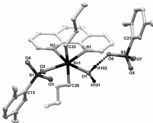
Figure 1. Molecular structure of 3 shown at the 50% ellipsoidal probability level. One of the sulfonate anions is bound to tin, while the other is involved in a \text{O}-\text{H}\cdots\text{O} hydrogen bonding with the coordinated water proton. All the hydrogen atoms (except those of the coordinated water) have been removed for the sake of clarity.
