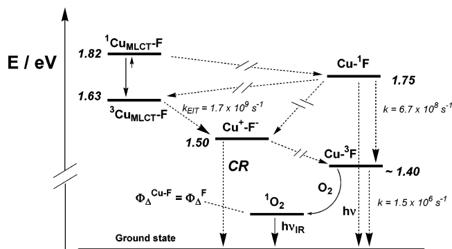
Figure 6. Energy level diagram for F-Cu-F and related photoinduced processes upon excitation of both chromophores. In the shorthand notations, only one F unit is indicated for F-Cu-F because under our experimental conditions, i.e., light intensity, only one F unit can be excited. The excited state energies of ^3\text{CuMLCT-F} and \text{Cu-}^1\text{F} are estimated from the 77 K emission band maxima of Cu and F , respectively, that of ^1\text{CuMLCT-F} is located 1500\text{ cm}^{-1} above ^3\text{CuMLCT-F} (ref 38), and that of \text{Cu-}^3\text{F} from theoretical calculations (ref 8). The position of the CS state is obtained from the electrochemical data.
