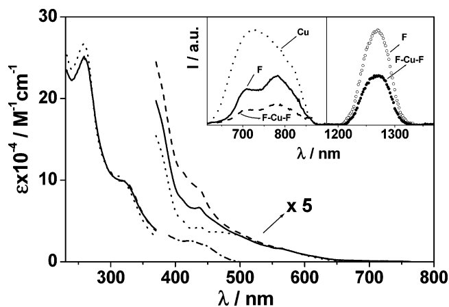
Figure 5. Absorption spectrum of F-Cu-F in CH 2 Cl 2 (—) and benzonitrile (---), compared to the sum spectrum of 2 F + Cu (····) in CH 2 Cl 2 ; the profile obtained by subtracting the sum spectrum to the experimental one is (---). Inset: emission spectra in CH 2 Cl 2 ; fullerene fluorescence and MLCT band (left), sensitized singlet oxygen luminescence (right), \lambda_{exc} = 600 nm, A = 0.190 for all samples, light partitioning in F-Cu-F is 0.5:1:0.5. The emission properties of F are the same as for 9 .
