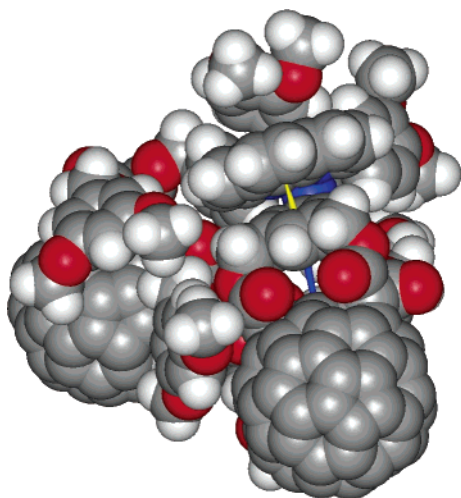
Figure 4. Snapshot of the theoretical structure of F-Cu-F at 300 K obtained from a Molecular Dynamics calculation showing the fullerene-phenyl-phenanthroline-phenyl stacking (the dodecyloxy groups have been replaced by methoxy substituents for clarity). The shortest distance between the fullerene sphere and its bridging phenyl ring (blue line) is 4.3 Å; the distance from the center of the phenyl ring of one ligand to the center of the central six-membered ring of the phenanthroline of the other ligand (yellow line) is 3.9 Å.
