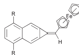
21 , R = H; \mu 3.37 D 22 , R = OMe; \mu 2.92 D
