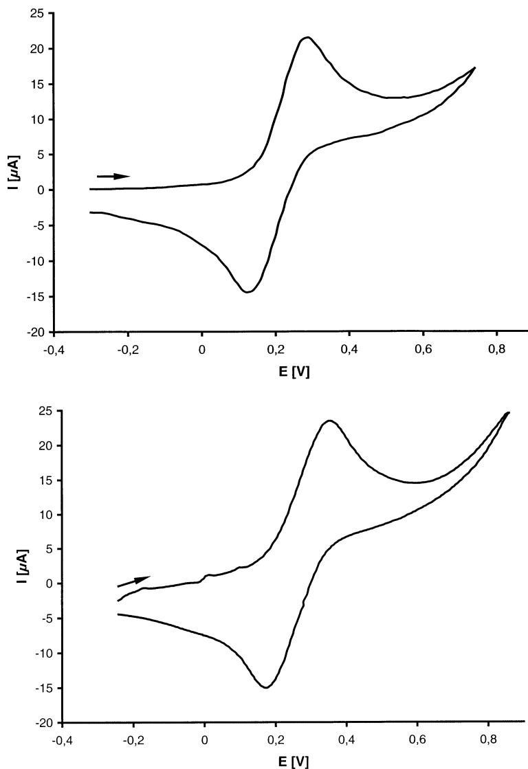
Fig. 1. Cyclic voltammograms of 3 (top) and 5 (bottom) in tetrahydrofuran solutions at 25 °C.
