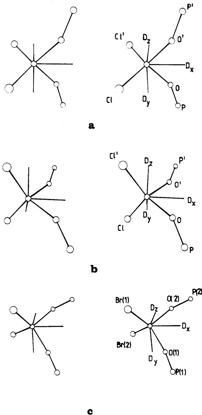
Figure 5. (a and b) Stereoscopic drawings for the two magnetically different zinc tetrahedra in the unit cell of \text{ZnCl}_2(\text{OPPh}_3)_2 . The D -tensor axes of one Mn(II) ion are superimposed on both tetrahedra. (c) Stereoscopic drawing of the zinc tetrahedron for \text{ZnBr}_2(\text{OPPh}_3)_2 with D -tensor axes of Mn(II) ion superimposed.
