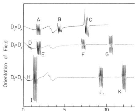
Figure 2. X-Band spectra (9.515 GHz) of Zn(Mn)Br 2 (OPPh 3 ) 2 with field along the three principal axes of the D tensor found experimentally as D 1 , D 2 , and D 3 and assigned to D y , D z , and D x , respectively, of the Hamiltonian in ref 3 (label for horizontal axis should read field/kG).
