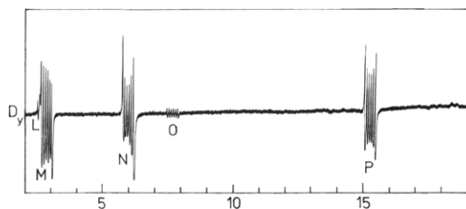
Figure 3. Q-Band spectrum (35.55 GHz) of Zn(Mn)Br 2 (OPPh 3 ) 2 with field close to the D y principal axis. (label for horizontal axis should read field/kG).
