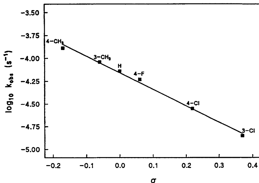
Figure 2. Hammett plot for the reaction of p -nitrophenyl- N - x -phenylsulphamates ( 1 \times 10^{-4} \text{ mol dm}^{-3} ) with cyclopentylamine ( 0.15 \text{ mol dm}^{-3} ) in 50% (v/v) aqueous acetonitrile at 37^\circ\text{C}
