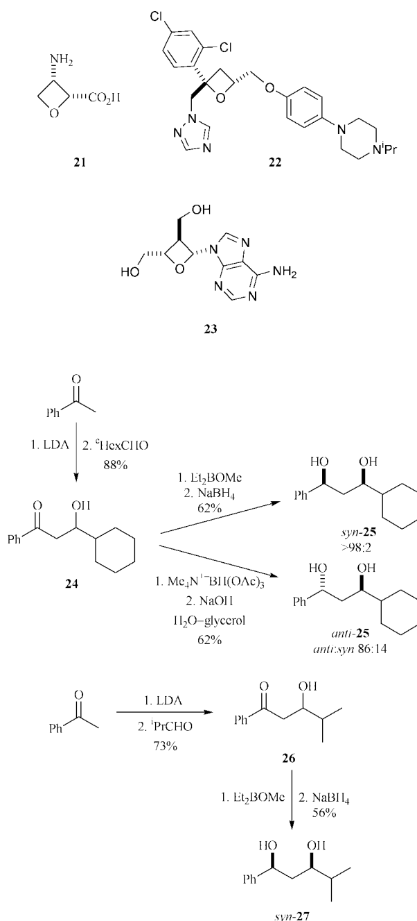
Scheme 5
