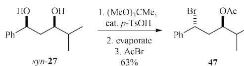
Scheme 10
