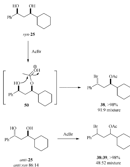
Scheme 12
