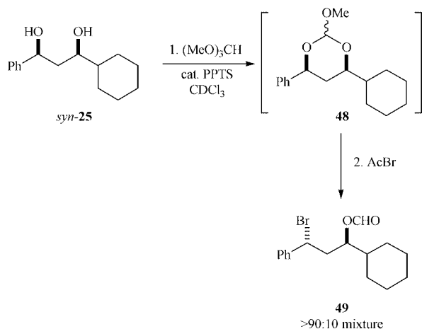
Scheme 11
