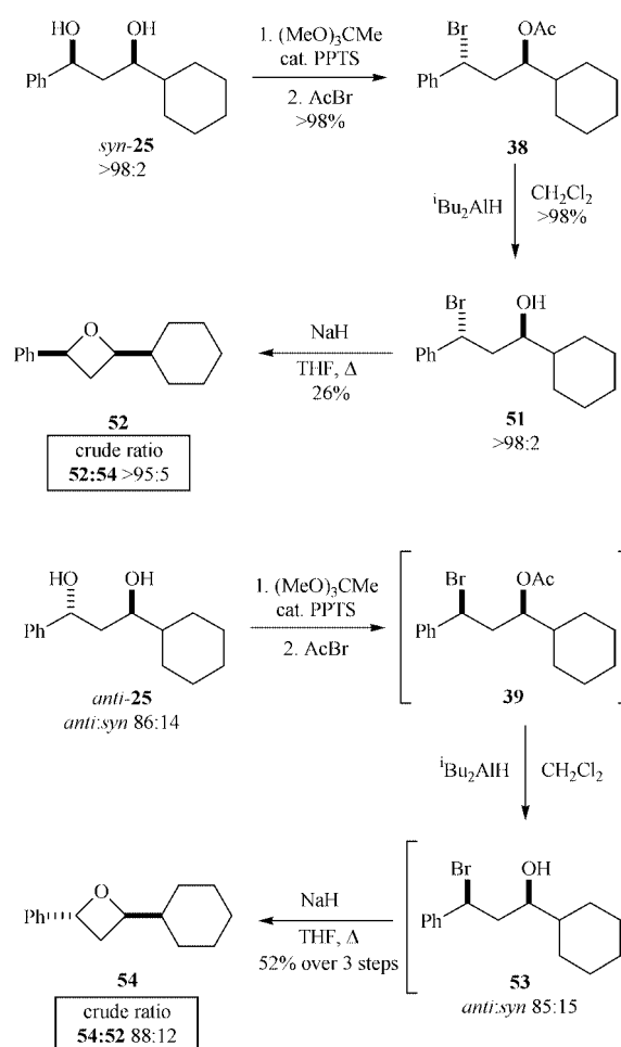
Scheme 13
