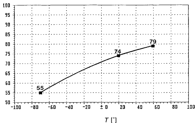
Fig. 2. Temperature dependence of the diastereoisomeric ratio (2R,3'S)\text{-2e}/(2S,3'S)\text{-2e} in the Paterno-Büchi reaction
