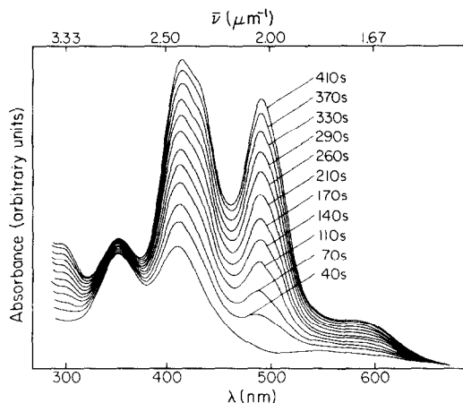
Fig. 3. Electronic spectral changes in a 12 M HCl solution originally 6.7 \times 10^{-3} M in \text{IrCl}_6^{3-} on 254 nm irradiation.
