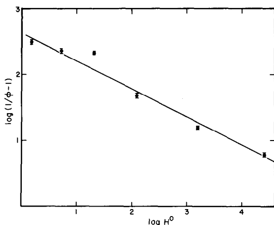
Fig. 4. Stern-Volmer plot based on quantum yields for photo-oxidation of \text{IrCl}_6^{3-} at various proton activities H^+ ( \Phi 254 nm) in HCl solutions: 12.0 M, 0.28; 9.0 M, 0.127; 6.0 M, 0.0411; 4.0 M, 0.00921; 2.0 M, 0.00868; 1.0 M, 0.00653).
