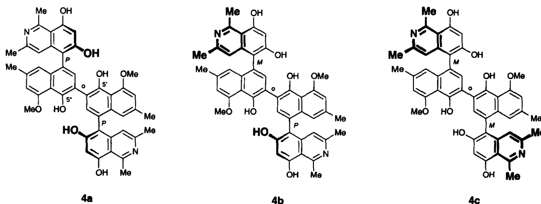
Fig. 2. Possible stereoisomeric forms of octadehydromichellamines ( 4 ).
