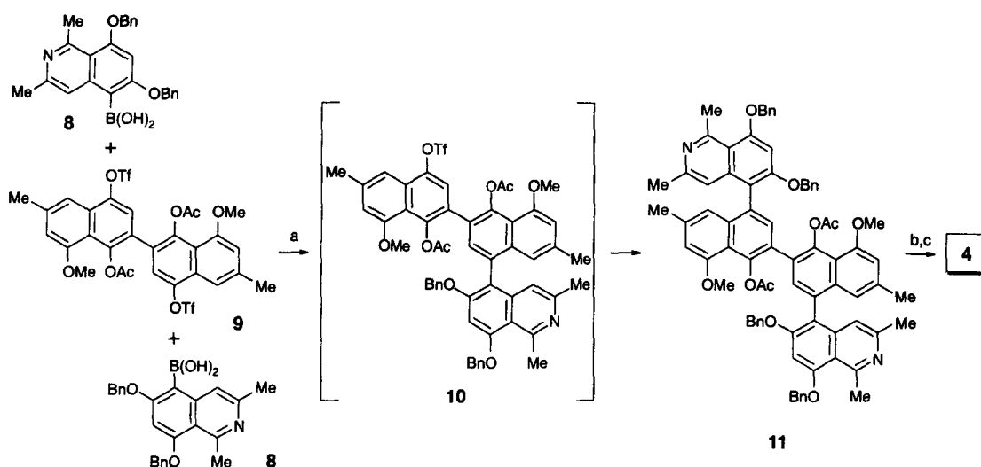
Scheme 2. Reagents and conditions: a) \text{Pd}(\text{PPh}_3)_4 , t\text{-BuOK} , \text{H}_2\text{O} / \text{DME} (1:3), 85^\circ\text{C} , 12%; b) \text{HCl} , \text{MeOH} , reflux; c) palladium black, \text{MeOH} / \text{HCO}_2\text{H} (2:3), reflux, 71%.
