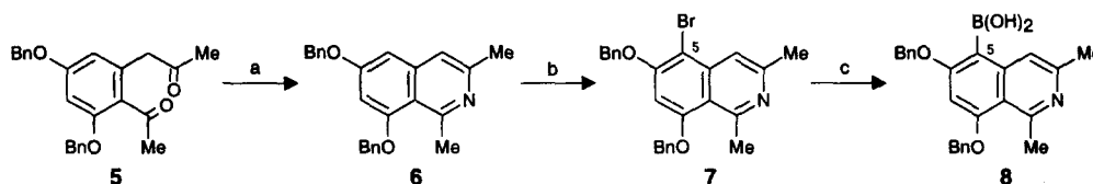
Scheme 1. Reagents and conditions: a) \text{NH}_4\text{OAc} , EtOH, 4 °C, 79%; b) \text{Br}_2 , NaOAc, \text{CH}_2\text{Cl}_2 , 25 °C, 93%; c) t -BuLi, THF / \text{Et}_2\text{O} (4:1), \text{B}(\text{OMe})_3 , -100 °C, 48%.
