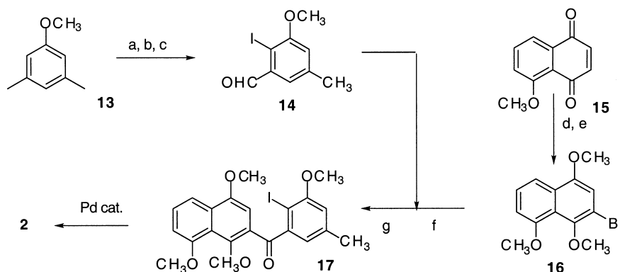
Scheme 3. Convergent synthesis of kinafluorenone: (a) \text{CCl}_4 , NBS, then \text{K}_2\text{CO}_3 , dioxane, 40%; (b) n\text{BuLi} , hexanes, \text{I}_2 -78^\circ\text{C} , 80%; (c) \text{COCl}_2 , DMSO, 95%; (d) \text{Na}_2\text{S}_2\text{O}_4 , ether then \text{Me}_2\text{SO}_4 , \text{K}_2\text{CO}_3 85%; (e) \text{CCl}_4 , \text{Br}_2 99% then \text{K}_2\text{CO}_3 , \text{Me}_2\text{SO}_4 60%; (f) t\text{BuLi} , ether, -78^\circ\text{C} (quant.); (g) PCC, \text{CH}_2\text{Cl}_2 , 80%
