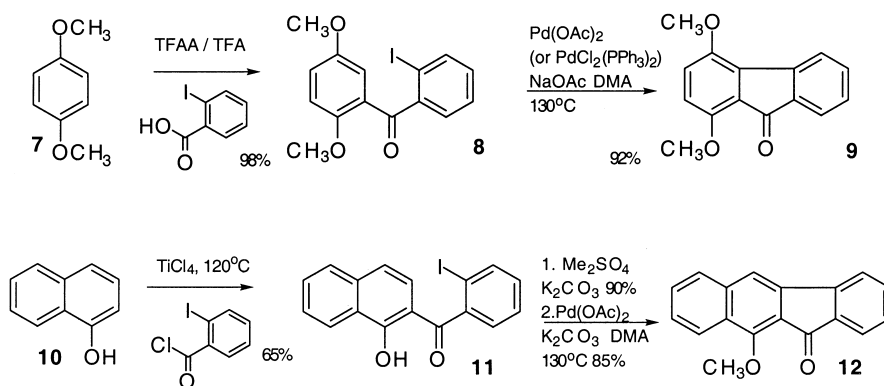
Scheme 2. Model arylation route to benzo[ b ]fluorenones
