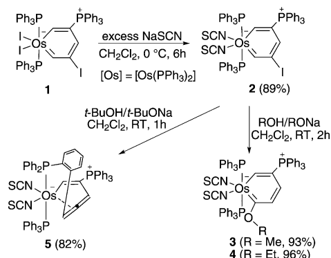
Scheme 2. Preparation of osmabenzene 2 and the reactions of compound 2 with alcohols.
