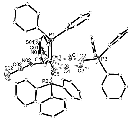
Figure 3. Molecular structure of compound 5 . Ellipsoids set at 50% probability. The hydrogen atoms of the PPh 3 groups are omitted for clarity.
