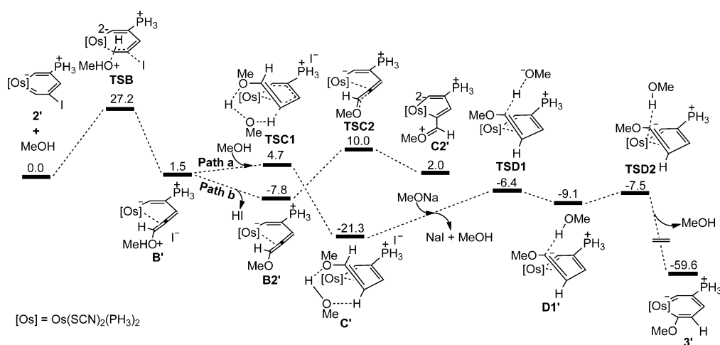
Figure 5. Calculated energy profile for the formation of structure 3' , based on the reaction mechanism shown in Scheme 6. The relative electronic energies are given in kcal mol -1 .
