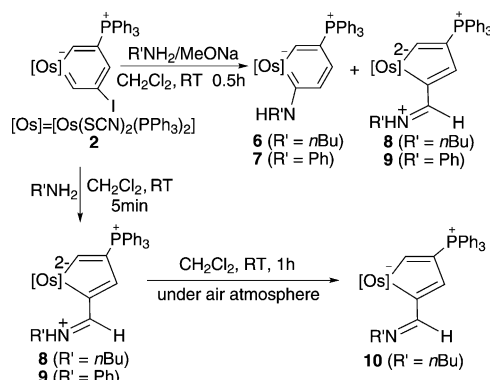
Scheme 3. Reactions of osmabenzene 2 with amines.
