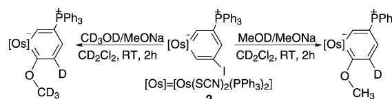
Scheme 4. Reactions of osmabenzene 2 with deuterium-labeled MeOH.
