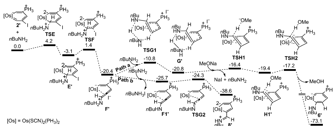
Figure 6. Calculated electronic energy profile for the formation of structures 6' and 8' , based on the reaction mechanism shown in Scheme 6. The relative electronic energies are given in kcal mol -1 .
