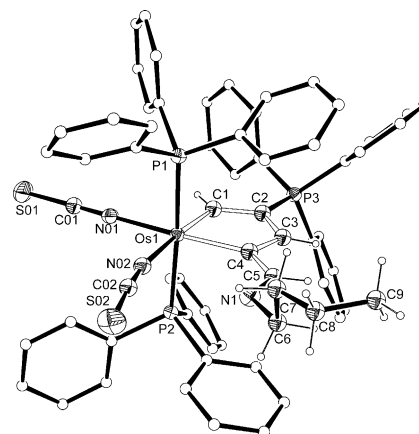
Figure 4. Molecular structure of compound 10 . Ellipsoids set at 50% probability. The hydrogen atoms of the \text{PPh}_3 groups are omitted for clarity.
