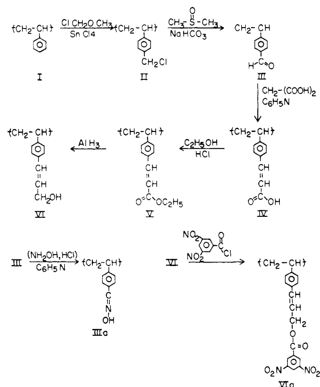
Scheme II. Preparation of the Solid Support
