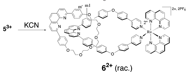
Scheme 3. Demetalation of 5^{3+} Using KCN
