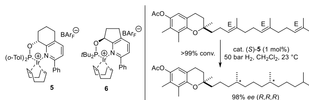
Scheme 2. Examples of pyridine-based iridium complexes and application of complex (S)- 5 in the hydrogenation of \gamma -tocotrienyl acetate.
