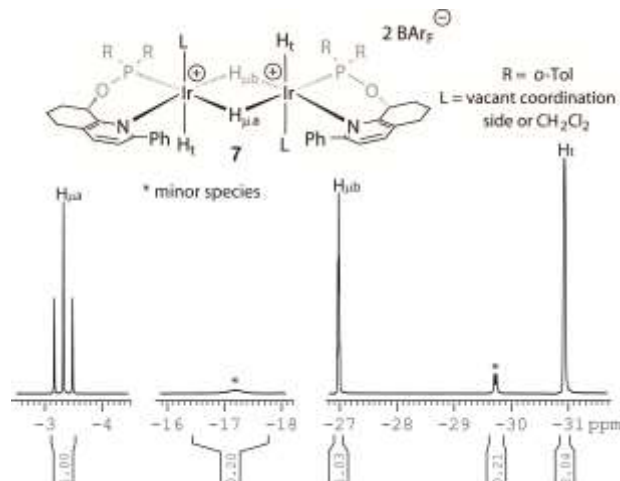
Figure 1. Section of the hydride region showing the hydrides signals of the dinuclear iridium hydride complex 7 and the minor species (*), respectively ( R = o\text{-Tol} , L = \text{CD}_2\text{Cl}_2 ; 295 K, 500 MHz, \text{CD}_2\text{Cl}_2 ).
