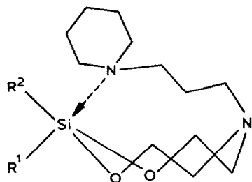
Fig. 2. Possible conformer of N -piperidinopropyl-dioxazasilacyclooctanes.
