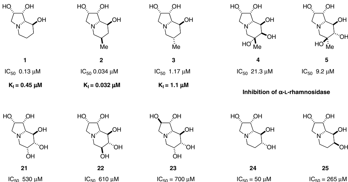
Figure 2. IC 50 (μM) of naringinase inhibition by L-swainsonine analogues.
