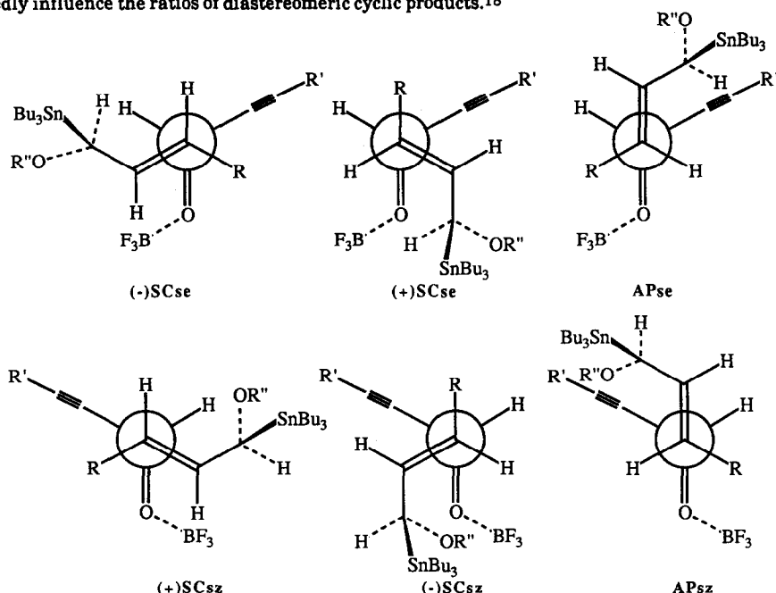
Figure 4. Newman projections of transition states for \text{BF}_3 promoted, syn selective additions of (R) - \alpha -alkoxyallylstannanes to 2-alkynals (acyclic; \text{R} = \text{R}' = \text{Bu} , \text{R}'' = \text{BOM} ; cyclic; \text{R}, \text{R}' = \text{ring} ; \text{R}'' = \text{MOM} ). SC = synclinal, AP = antiperiplanar; (+) / (-) refers to the relationship between the \text{C}=\text{C} and the \text{C}=\text{O} .
