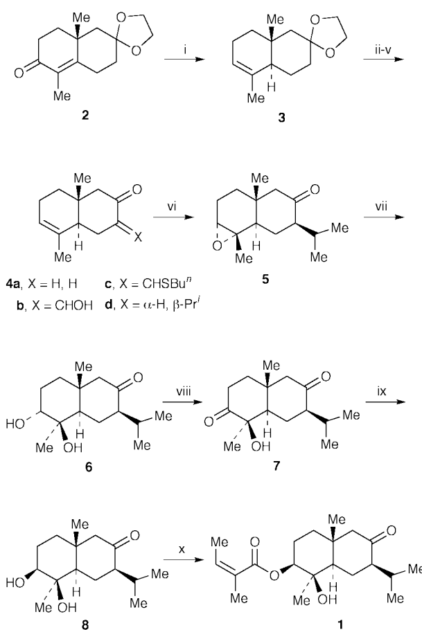
Scheme 1 Reagents and conditions: i, Li, NH 3 , THF- t -BuOH; CIPO-(OEt) 2 ; Li, MeNH 2 (61%); ii, AcOH-H 2 O (95%); iii, NaH, HCO 2 Et, Et 2 O; iv, n -BuSH, p -TsOH, benzene (90%, 2 steps); v, LiMe 2 Cu, Et 2 O (99%); vi, m -ClC 6 H 4 CO 2 H, Na 2 CO 3 , CH 2 Cl 2 (93%); vii, H 2 SO 4 , Me 2 CO-H 2 O (40%); viii, C 5 H 5 N·SO 3 , Et 3 N, DMSO (91%); ix, Zn(BH 4 ) 2 , DME (70%); x, ( Z )-MeC=C(Me)CO 2 COC 6 H 4 Cl 3 , DMAP, PhMe (74%).
