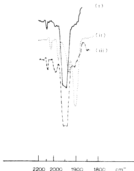
Fig. 2. Infrared spectra of \text{Mo}_2(\text{CO})_{10}(\text{dppp}) in toluene (i) at 25°C, (ii) 24 h reflux under \text{N}_2 and (iii) 24 h reflux under CO.
