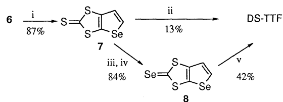
Scheme 2. Reagents and conditions: i, DDQ, toluene, reflux, 20 h; ii, P(OMe) 3 , reflux, 2 h; iii, (MeO) 2 SO 2 , 80 °C, 0.5 h, then aq. HBF 4 ; iv, NaBH 4 , Se, EtOH, rt, 0.5 h; v, P(OMe) 3 , benzene, reflux, 1 h.
