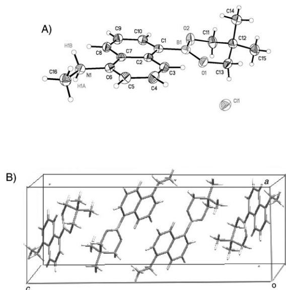
Figure 3. A) The crystal structure of compound 10 -HCl; [14] B) packing diagram for molecules in the unit cell.
