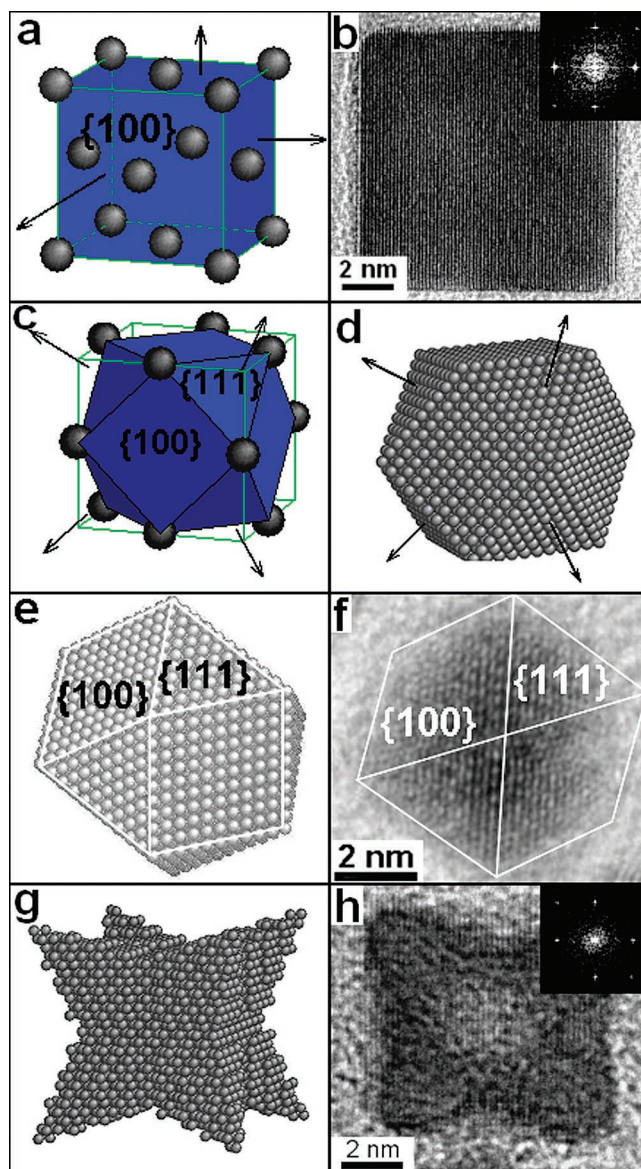
Figure 3. Growth mechanism on {1,0,0} and {1,1,1} facets. (a and b) Models showing the growth on the {1,0,0} facet of platinum to form faceted platinum nanocubes. (c–e) Models showing the octapod unit cell, HRTEM image of a typical faceted platinum nanocube. (d, e, and g) Models showing truncated octahedral nuclei and growth in the {1,1,1} facets. (f) HRTEM of truncated octahedral nuclei. (h) HRTEM image of a filled octapod nanocube.
