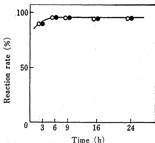
Fig. 4. Time Course of Methylation of Compounds 2 and 3 with Diazomethane
