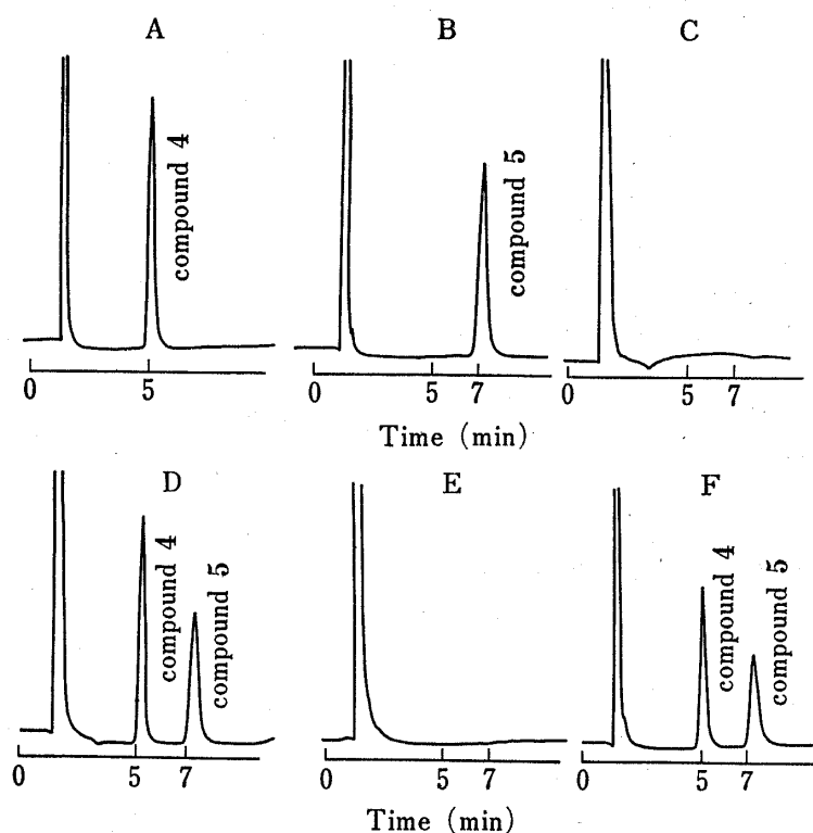
Fig. 6. Chromatograms of Compounds 4, 5 and Extracts from Human Whole Blood and Urine with or without Addition of Compounds 1 and 3
