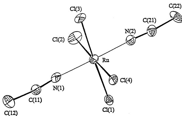
Fig. 2. ORTEP (k) plot of the molecular structure of 2 . Selected bond lengths (Å) and angles (°) with estimated S.D. values in parentheses: Ru–N(1) 2.024(7), Ru–N(2) 2.016(7), Ru–Cl(1) 2.338(7), Ru–Cl(2) 2.326(7), Ru–Cl(3) 2.368(6), Ru–Cl(4) 2.356(8), N(1)–Ru–N(2) 178(2), N(1)–Ru–Cl(1) 93.4(7), N(1)–Ru–Cl(2) 90.0(8), N(1)–Ru–Cl(3) 87.4(7), N(1)–Ru–Cl(4) 90.4(8), Cl(1)–Ru–Cl(2) 91.37(10), Cl(2)–Ru–Cl(3) 90.7(3), Cl(3)–Ru–Cl(4) 88.20(10), Cl(4)–Ru–Cl(1) 89.7(3).
