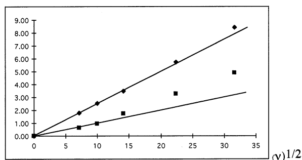
Fig. 6. Plot of anodic peak current density: i_p^a \text{ cm}^{-2} \times 100 , vs. (v)^{1/2} of \text{Ru}(\text{AN})_3\text{Cl}_3 ( 3 ) 6.6 \times 10^{-4} \text{ M} in acetonitrile. Lower line: CV at 133 mV; upper line CV at 1840 mV. Each scanned at 50, 100, 200, 500 and 1000 \text{mV s}^{-1} .
