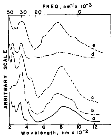
Figure 3. Electronic spectra of (a) Cu(tfacMeDPT), (b) Cu(acacMeDPT), (c) Cu(benacMeDPT), (d) Cu(benacDPT), and (e) Cu(tfacPhDPT) 10^{-3} M in \text{C}_2\text{Cl}_4 (low-energy region) and 10^{-4} M in \text{CH}_3\text{OH} (high-energy region).
