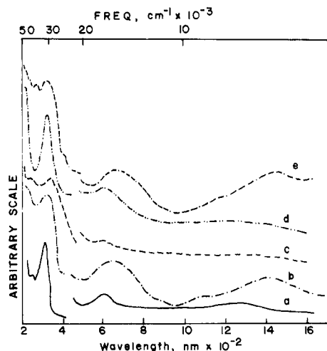
Figure 1. Electronic spectra of (a) Ni(tfacMeDPT), (b) Ni(acacMeDPT), (c) Ni(benacDPT), (d) Ni(benacMeDPT), and (e) Ni(tfacPhDPT) 10^{-3} M in C 2 Cl 4 (low-energy region) and 10^{-4} M in CH 3 OH (high-energy region)).
