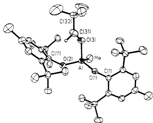
Figure 1. Structure of \text{AlMe(BHT)}_2[\text{O}=\text{C(H)Bu}] (1). Thermal ellipsoids are drawn at the 30% level, and the hydrogen atoms [except that bonded to C(31)] are omitted for clarity.
