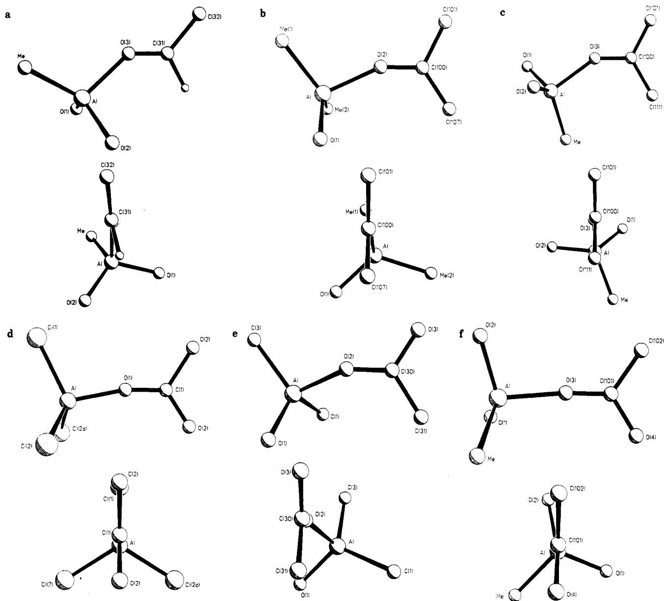
Figure 4. Partial coordination spheres of the organic carbonyl ligands for 1 (a), 8 (b), \text{AlMe(BHT)}_2(\text{O}=\text{CPh}_2) (c), \text{AlCl}_3[\text{O}=\text{C(Me)OPh}] (d), \text{AlEt}_2(\text{BHT})[\text{O}=\text{C(OMe)C}_6\text{H}_4\text{-p-Me}] (e), and 17 (f), viewed perpendicular and parallel to the \text{C}=\text{O} vector.
