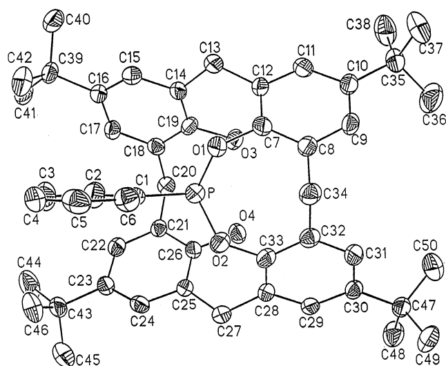
Fig. 1. Molecular structure of [(\text{PhPC})_2\text{H}_2] ( 2 ), showing the atom labelling scheme.
