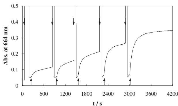
Figure 2. Successively measured absorbance (at 664 nm) vs time profile for a LMB solution (10 \mu\text{M} , pH 2) added ( \uparrow ) with various concentrations of Cr(VI) (left to right; 1, 1.96, 3.77, 7.02, and 12.3 \mu\text{M} ) in the presence of AA (120 ppm). The abrupt rise of the absorbance was caused by an instrumental perturbation when visible light was irradiated ( \downarrow ) from an external lamp to regenerate LMB. The absorbance dropped back to a normal level when the light was off.
