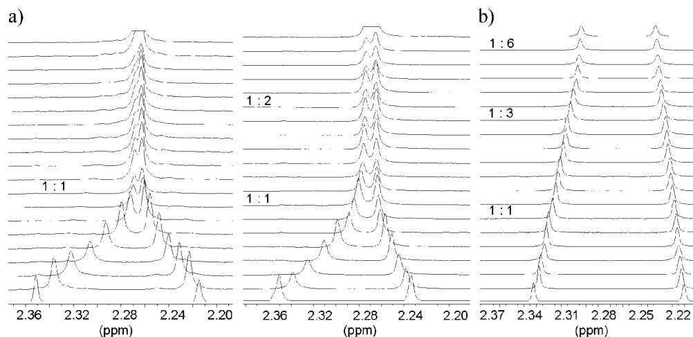
FIGURE 3. (a) Partial 1 H NMR spectra (400 MHz) of receptor 1 after addition of (from bottom to top) 0.00–2.49 equiv of α-glucopyranoside 3a ([ 1 ] = 1.02 mM): left, CDCl 3 ; right, water-containing CDCl 3 (0.04% H 2 O). (b) Partial 1 H NMR spectra (500 MHz, CDCl 3 ) of receptor 10 after addition of 0.00–7.25 equiv of 3a ([ 10 ] = 0.70 mM). Shown are chemical shifts of the pyridine methyl groups.
