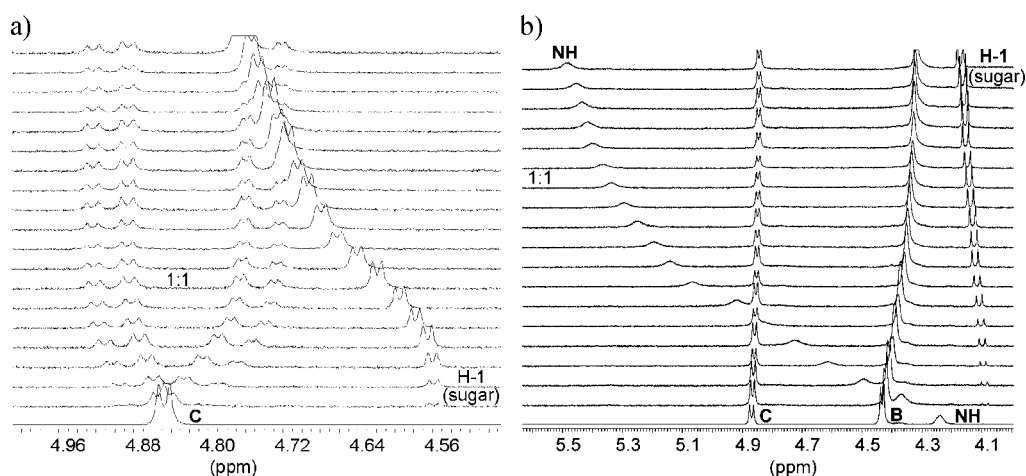
FIGURE 4. Partial 1 H NMR spectra (400 MHz; CDCl 3 ) of receptor 1 after addition of (a) 0.00–2.67 equiv of α-glucopyranoside 3a ([ 1 ] = 0.86 mM) and (b) 0.00–1.80 equiv of β-galactopyranoside 4a ([ 1 ] = 0.90 mM).
