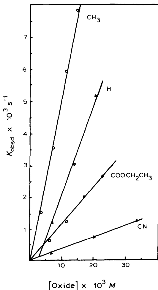
Fig. 1. Plot of k_{\text{obsd}} vs. (p\text{-RC}_6\text{H}_4)(\text{Me})_2\text{NO} concentration for reaction 3 in \text{CH}_2\text{Cl}_2 at 18.9^\circ\text{C} .
