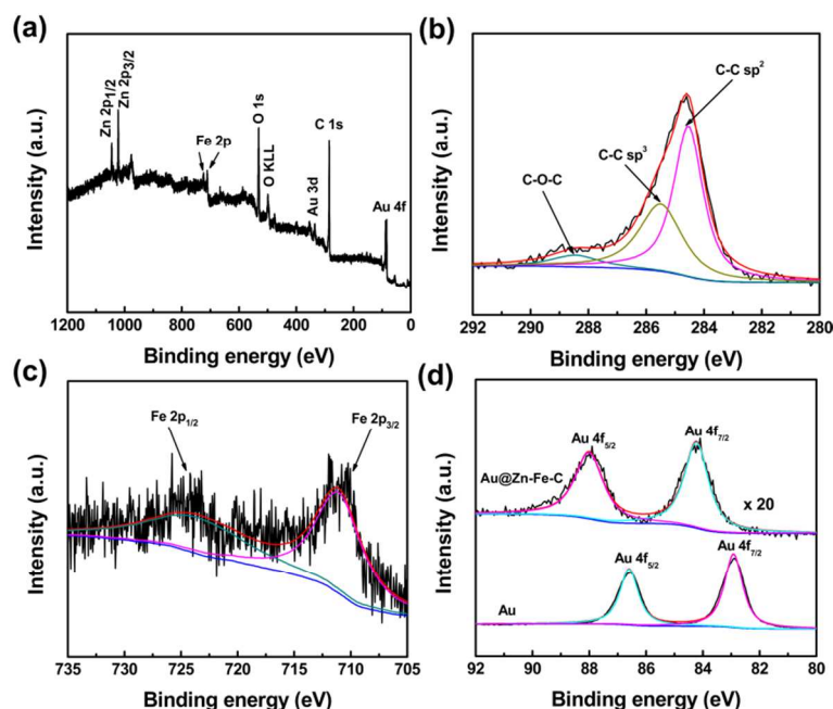
Figure 3. (a) XPS survey spectrum and high-resolution scans of (b) C1s, (c) Fe2p, and (d) Au4f electrons of the Au@Zn-Fe-C hybrids. The spectrum of the Au4f electrons of pure Au nanoparticles is also included in panel (d). Black curves are experimental data and colored curves are deconvolution fits.
