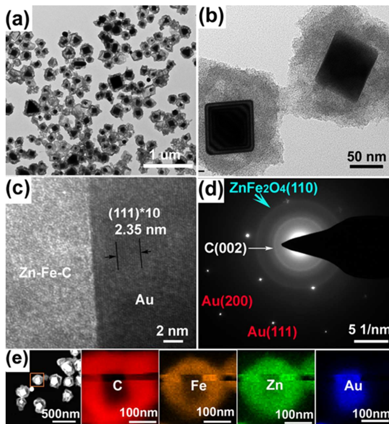
Figure 2. (a, b) Representative TEM, (c) HRTEM images, (d) the corresponding SAED patterns, and (e) EDX maps of Au@Zn-Fe-C hybrids.
