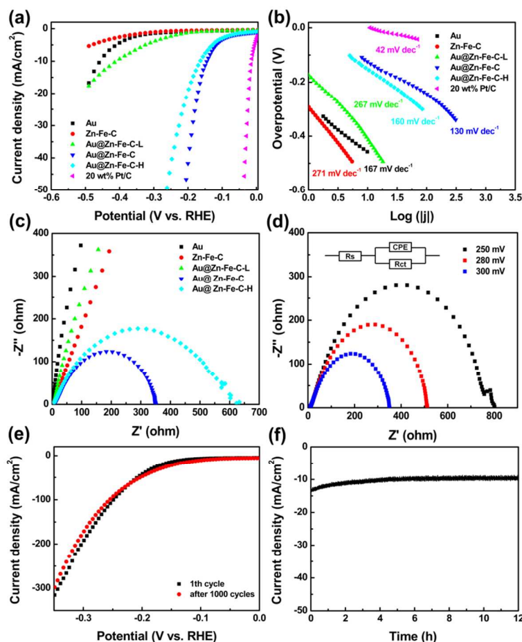
Figure 6. (a) Polarization curves and (b) corresponding Tafel plots of Au nanoparticles, Zn-Fe-C, Au@Zn-Fe-C-L, Au@Zn-Fe-C, Au@Zn-Fe-C-H and 20 wt% Pt/C at 5 \text{ mV s}^{-1} in a 0.5 \text{ M H}_2\text{SO}_4 solution (iR-corrected). (c) Electrochemical impedance spectra of various samples for HER at -0.3 \text{ V} . (d) Electrochemical impedance spectra of Au@Zn-Fe-C at various overpotentials for HER in 0.5 \text{ M H}_2\text{SO}_4 . Inset shows the equivalent circuit, where R_s is the (uncompensated) electrode series resistance, CPE is the constant-phase element and R_{ct} is the charge-transfer resistance. (e) Polarization curves of Au@Zn-Fe-C before and after 1,000 cycles in stability test. (f) Time dependence of the HER current density of Au@Zn-Fe-C loaded on carbon cloth at -0.15 \text{ V} vs. RHE (iR-uncorrected).
