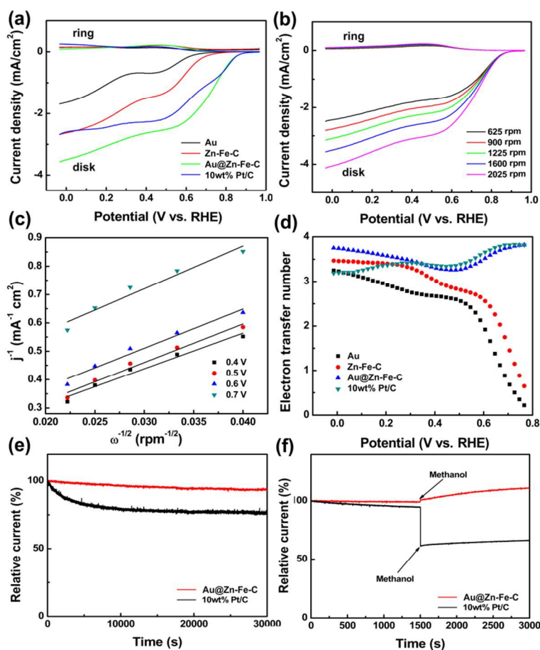
Figure 4. (a) RRDE voltammograms of Au nanoparticles, Zn-Fe-C, Au@Zn-Fe-C, and 10 wt% Pt/C at a rotation rate of 1600 rpm in an O 2 -saturated 0.1 M KOH solution at 10 mV s -1 . (b) RRDE voltammograms
