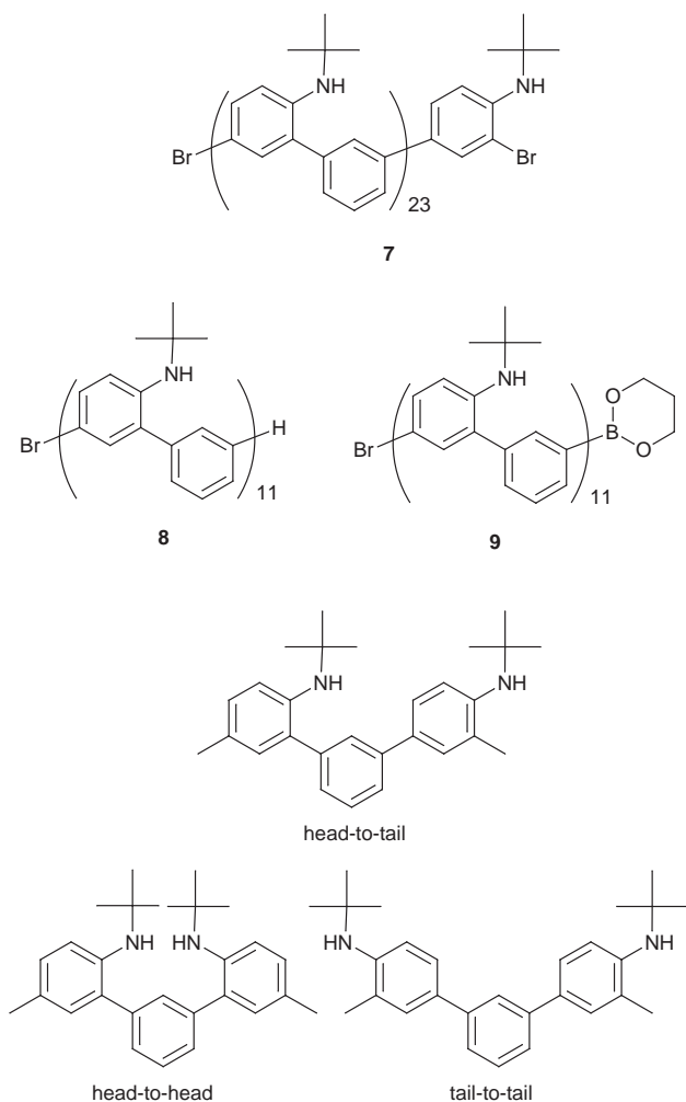
Fig. 2 Three kinds of connection between monomers in polymer 6 .
