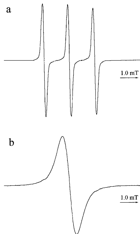
Fig. 3 EPR spectra in benzene at 20 °C: (a) 1 ; (b) 2 .
