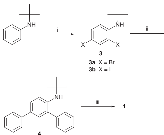
Scheme 1 Reagents and conditions: i, \text{BTMABr}_3 or \text{BTMAICl}_2 , \text{CaCO}_3 , \text{CH}_2\text{Cl}_2 – \text{MeOH} , room temp; ii, \text{C}_6\text{H}_5\text{B}(\text{OH})_2 , \text{Pd}(\text{PPh}_3)_4 , \text{K}_2\text{CO}_3 , benzene– \text{H}_2\text{O} , reflux; iii, 3- \text{ClC}_6\text{H}_4\text{CO}_3\text{H} , \text{CH}_2\text{Cl}_2 , room temp.
