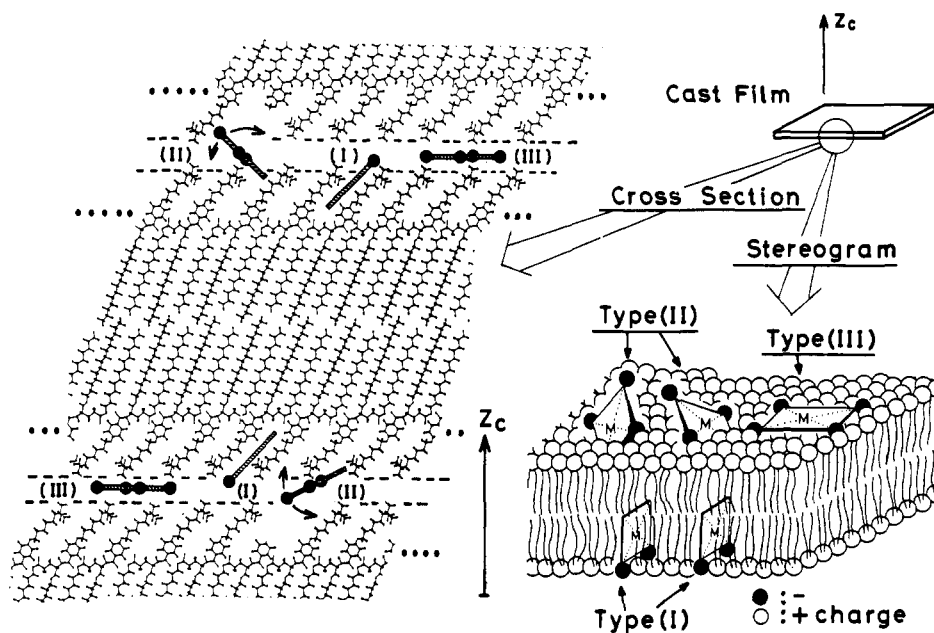
Figure 12. Schematic representation of three types of anionic porphyrins in a cast multibilayer film of 2C_{14}\text{-Glu-ph-C}_6\text{-N}^+ . The overall bilayer organization is assumed to be the same as that of Figure 3. For clarity, counterions are not shown and the bilayer units are separated from each other. The spacer portion is also not shown in "Stereogram". Type I porphyrins are inserted into the bilayer along the molecular axis of the spacer chain. Type II porphyrins are randomly placed on the bilayer surface. Type III porphyrins lie flat on the bilayer.
