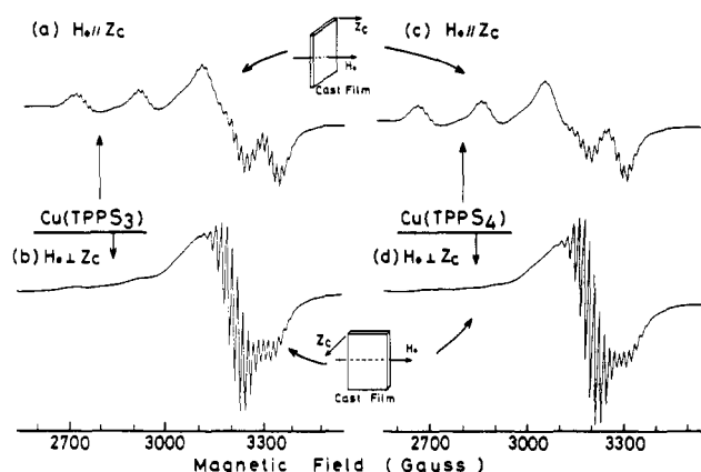
Figure 14. Observed ESR spectra of \text{Cu(TPPS}_3\text{)} and \text{Cu(TPPS}_4\text{)} in a cast film of \text{C}_8\text{-Azo-C}_{10}\text{-N}^+ : room temperature; [\text{porphyrin}]:[\text{C}_8\text{-Azo-C}_{10}\text{-N}^+] = 1:80 ; \nu = 9.222 GHz. Key: (a) and (b) \text{Cu(TPPS}_3\text{)} , (c) and (d) \text{Cu(TPPS}_4\text{)} .
