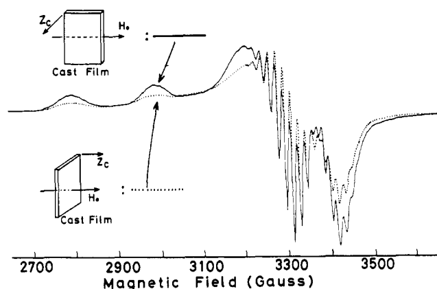
Figure 13. Observed ESR spectra of \text{Cu(ChP)} embedded in a cast multibilayer film of \text{C}_8\text{-Azo-C}_{10}\text{-N}^+ : room temperature; \nu = 9.4554 GHz; [\text{Cu(ChP)}]:[\text{C}_8\text{-Azo-C}_{10}\text{-N}^+] = 1:80 . Key: —, \Phi = 90^\circ ; ---, \Phi = 0^\circ .
