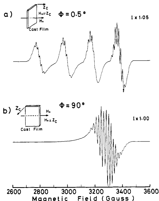
Figure 10. Most satisfactory simulation spectra obtained at \theta = 0.5^\circ , \sigma = 15^\circ , g_\parallel = 2.192 , g_\perp = 2.050 , A_\parallel = 197 G, A_\perp = 20 G, A_N^\parallel = A_N^\perp = 14 G, \Delta L_\parallel = 10 G, \Delta L_\perp = 8 G, and \nu = 9.4377 GHz. Key: (a) \Phi = 0.5^\circ , (b) \Phi = 90^\circ .
