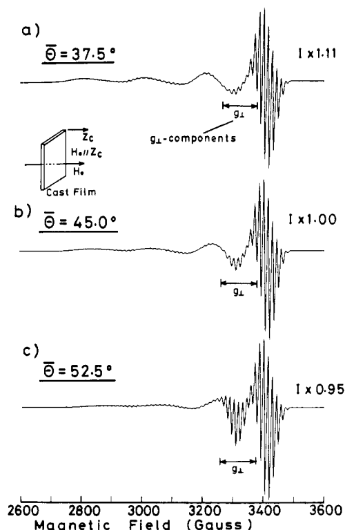
Figure 7. Influence of \bar{\theta} value on simulated spectra of Cu(PP) in a cast film at \Phi = 0.5^\circ and \sigma = 15^\circ . The other parameters are the same as those in Figure 8. Key: (a) \bar{\theta} = 37.5^\circ , (b) \bar{\theta} = 45.0^\circ , (c) \bar{\theta} = 52.5^\circ .
