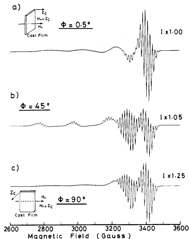
Figure 8. Most satisfactory simulation spectra obtained at \bar{\theta} = 0.5^\circ , \sigma = 15^\circ , g_{\parallel} = 2.192 , g_{\perp} = 2.050 , A_{\parallel} = 201 G, A_{\perp} = 28 G, A_{\parallel}^{\text{N}} = A_{\perp}^{\text{N}} = 14 G, \Delta L_{\parallel} = 9 G, \Delta L_{\perp} = 8 G (L's mean the peak to peak line-width parameter 34,39 ), and \nu = 9.455 GHz. Key: (a) \Phi = 0.5^\circ , (b) \Phi = 45^\circ , (c) \Phi = 90^\circ .
