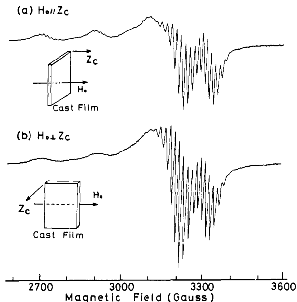
Figure 11. Observed ESR spectra of Cu(TPPS 3 ) embedded in a cast film of 2C 14 -Glu-ph-C 6 -N + : room temperature; \nu = 9.2210 GHz; [Cu(TPPS 3 )]:[2C 14 -Glu-ph-C 6 -N + ] = 1:80. Key: \Phi = 0^\circ , (b) \Phi = 90^\circ .
