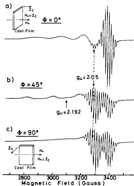
Figure 4. Observed ESR spectra of Cu(PP) embedded in a cast film of 2C_{14} -Glu-ph- C_6-N^+ : room temperature; \nu = 9.455 GHz; [Cu(PP)]: [2C_{14}\text{-Glu-ph-}C_6-N^+] = 1:58 . Key: (a) \Phi = 0^\circ , (b) \Phi = 45^\circ , (c) \Phi = 90^\circ .
