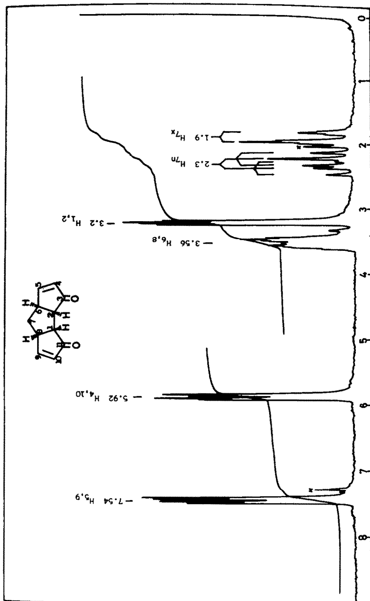
Fig. 1. ^1\text{H} NMR (100 MHz) spectrum of bis-enone 11a in \text{CDCl}_3 .
